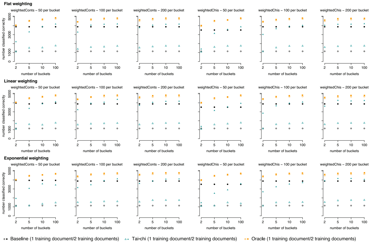
Figure 1: Test results. The rows from top to bottom show graphs for flat, linear and exponential weighting respectively. The three leftmost columns show graphs for feature selection based on weighted contingencies. The three columns at the right side show result graphs for feature selection based on weighted \chi^2 's. The first and fourth column have 50, second and fifth 100 and third and sixth column 200 examples per time bucket. The x-axis displays the number of buckets taken into account. The y-axis lists the number of examples classified correctly. Results are by displayed the amount of documents per bucket (2, 5, 10, 100). Cf. Section 4.1.
